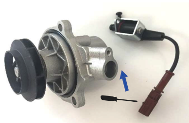
Waterpump A255 and A255E (mechanical version)
